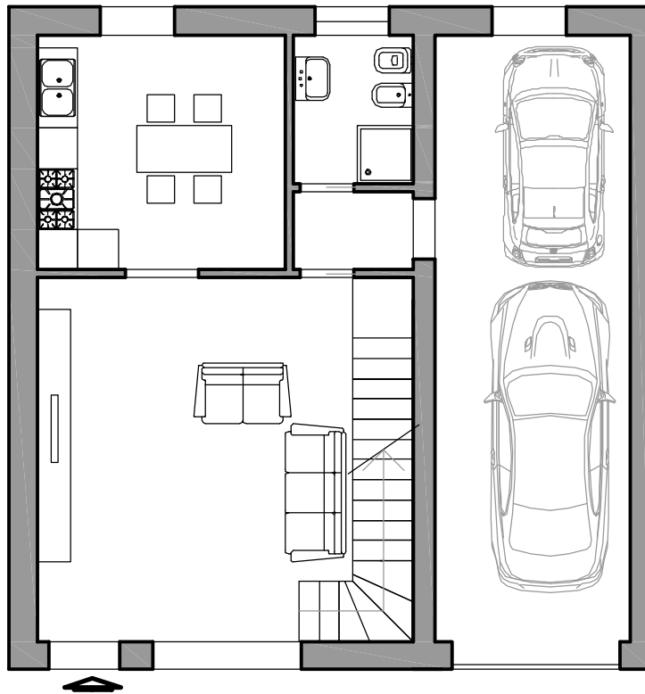
PIANO TERRA MQ 92
