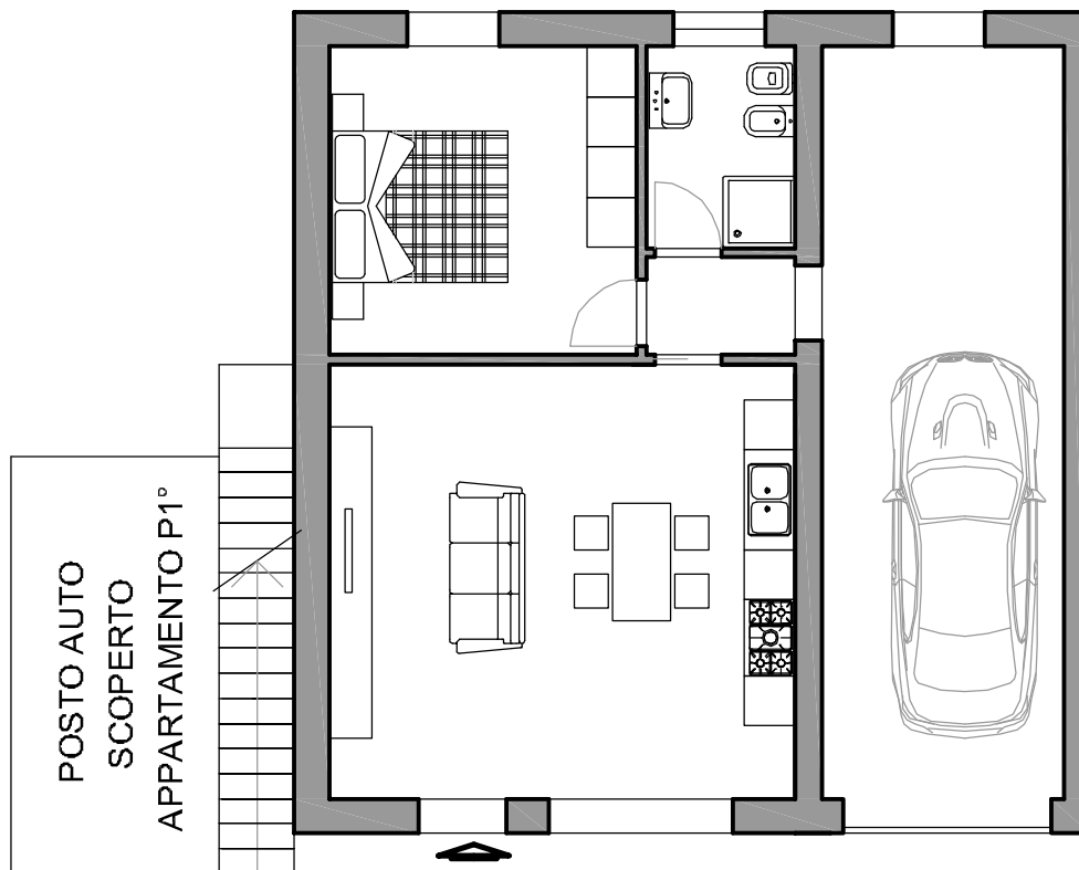
PIANO TERRA MQ 92
